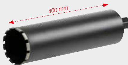
TRÉPAN DIAMANTÉ Ø 102 MM Concrete core drill Ø 102 mm
