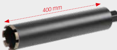
TRÉPAN DIAMANTÉ Ø 71 MM Concrete core drill Ø 71 mm
